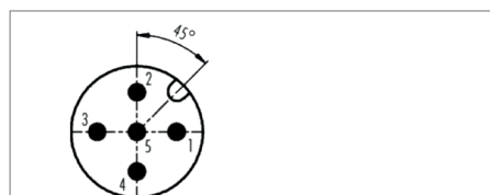
Pinout
